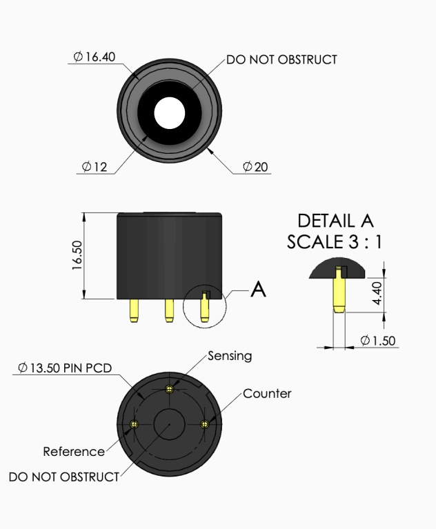
Product Dimensions All dimensions in mm All tolerances ±0.15 mm
