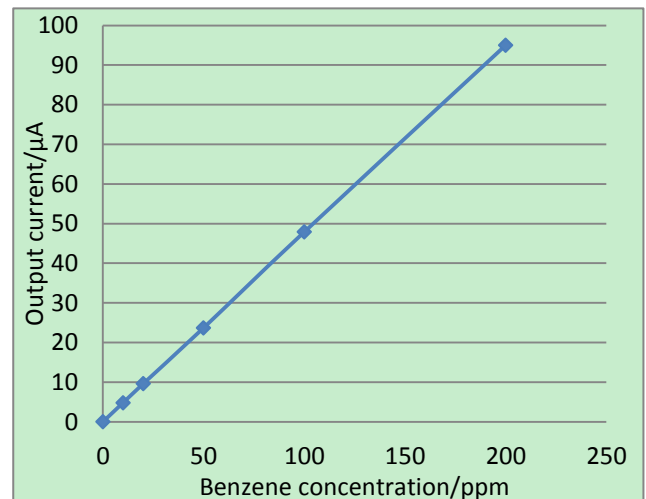
Fig4: Linearity
