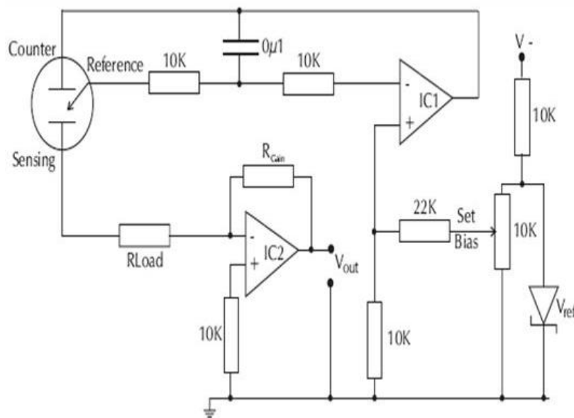
Fig2: ME4-C 6 H 6 test circuit
