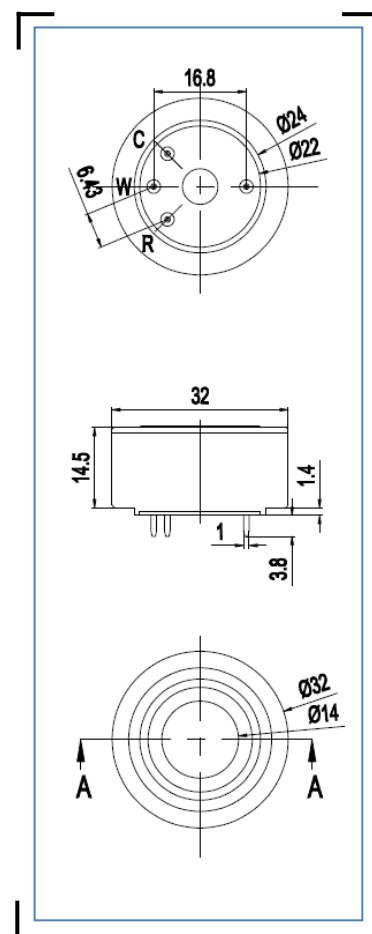
Fig1.Sensor Structure
