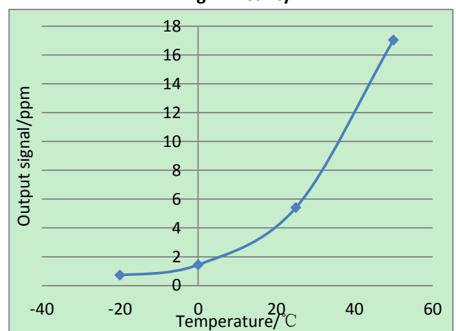
Fig6: Zero output of sensor at different temperature
